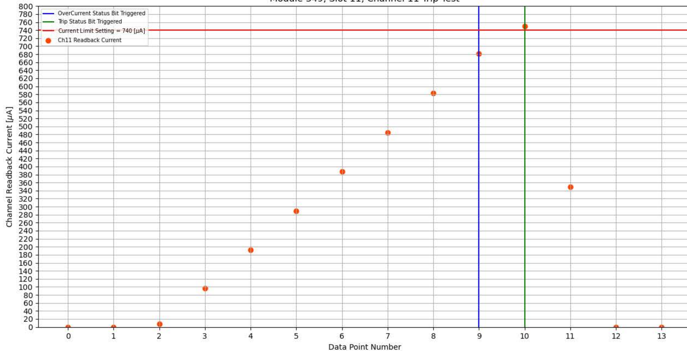
Module 349, Slot 11, Channel 11 Trip Test
