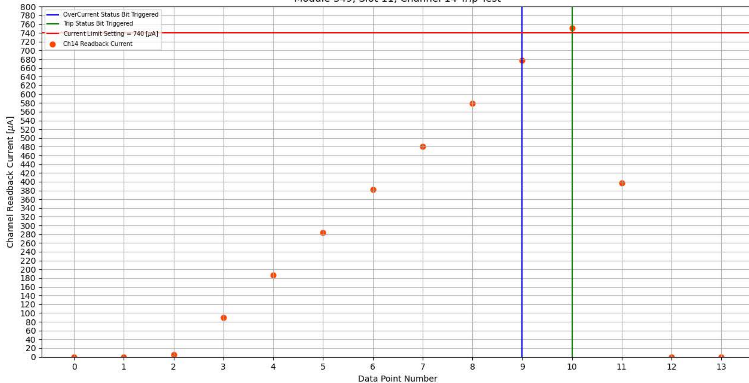
Module 349, Slot 11, Channel 14 Trip Test
