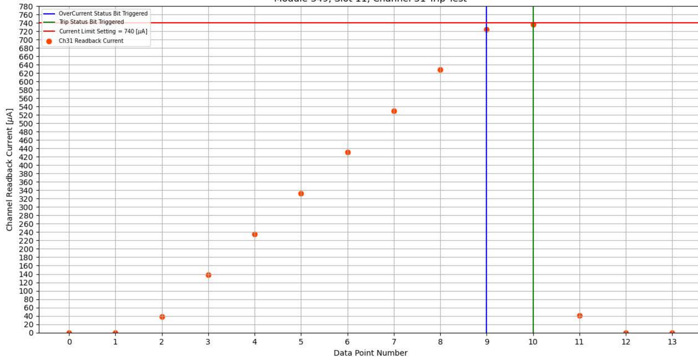
Module 349, Slot 11, Channel 31 Trip Test
