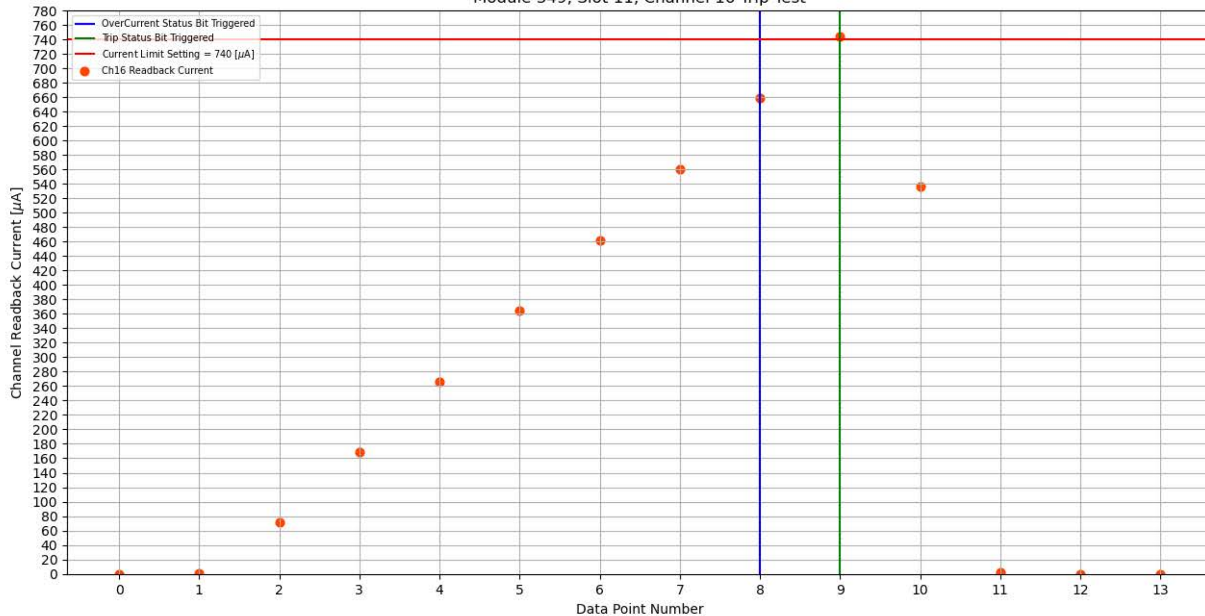
Module 349, Slot 11, Channel 16 Trip Test
