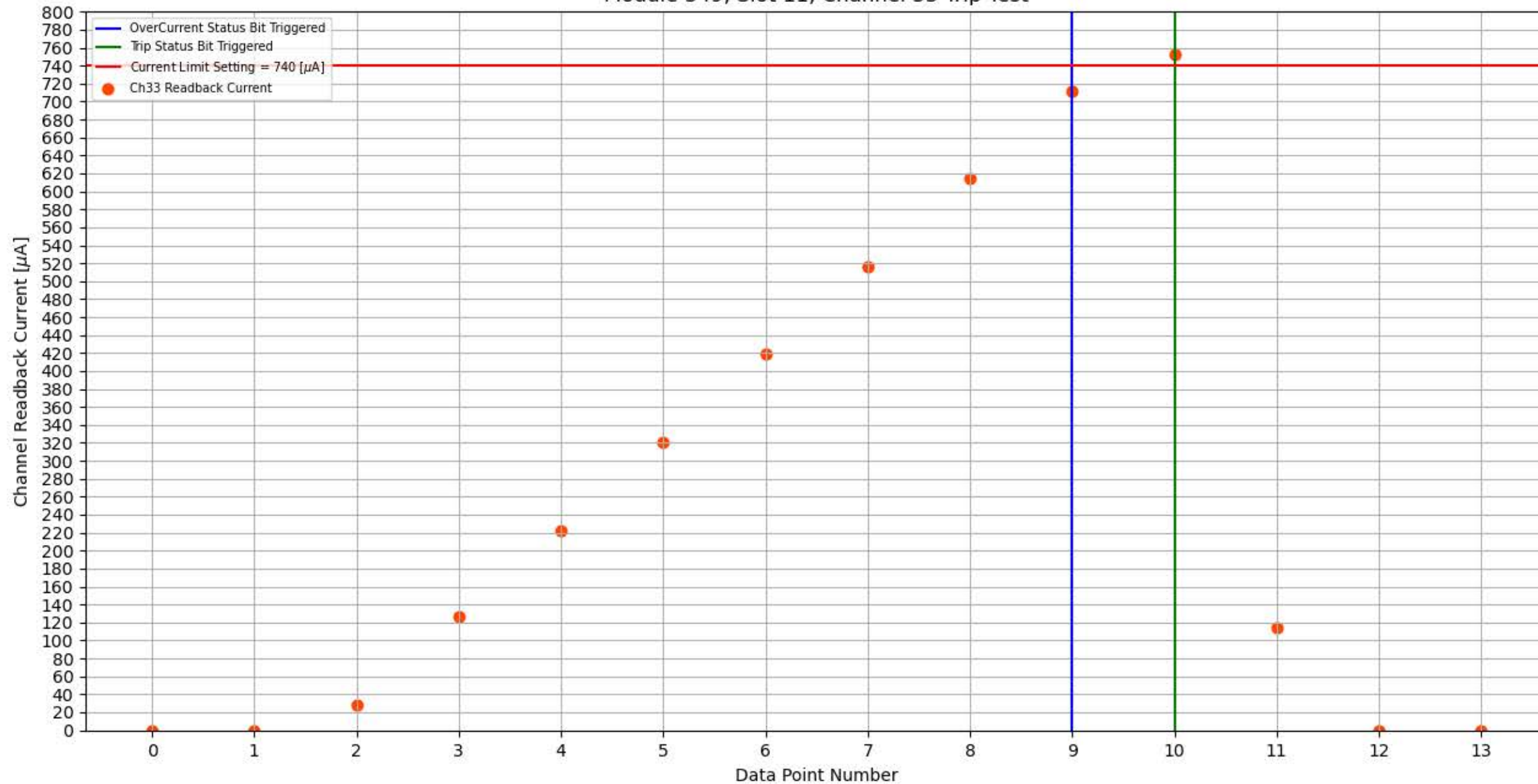
Module 349, Slot 11, Channel 33 Trip Test
