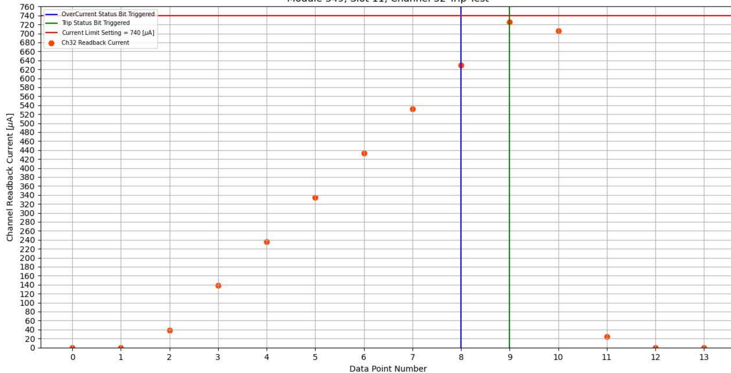
Module 349, Slot 11, Channel 32 Trip Test
