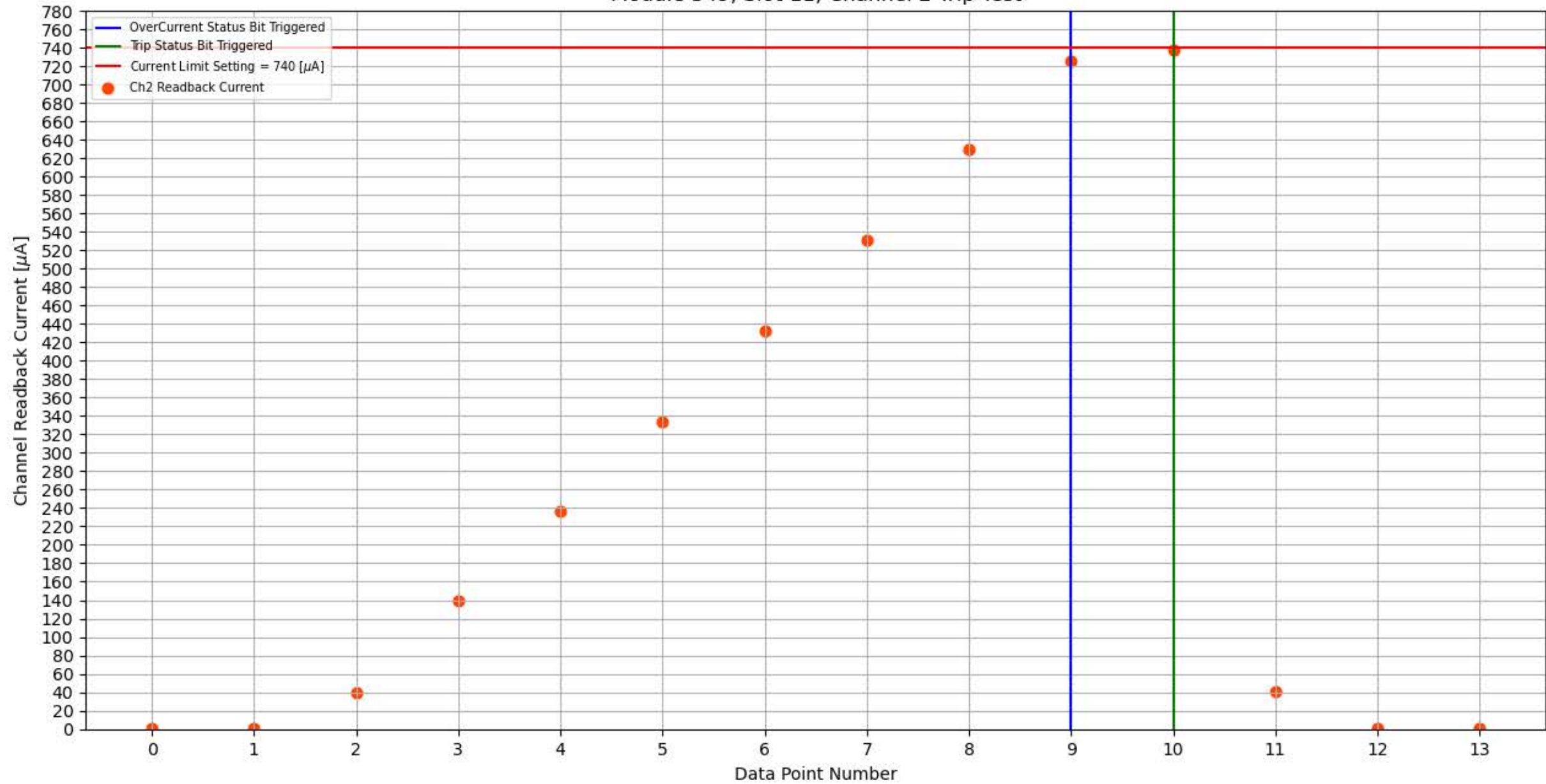
Module 349, Slot 11, Channel 2 Trip Test
