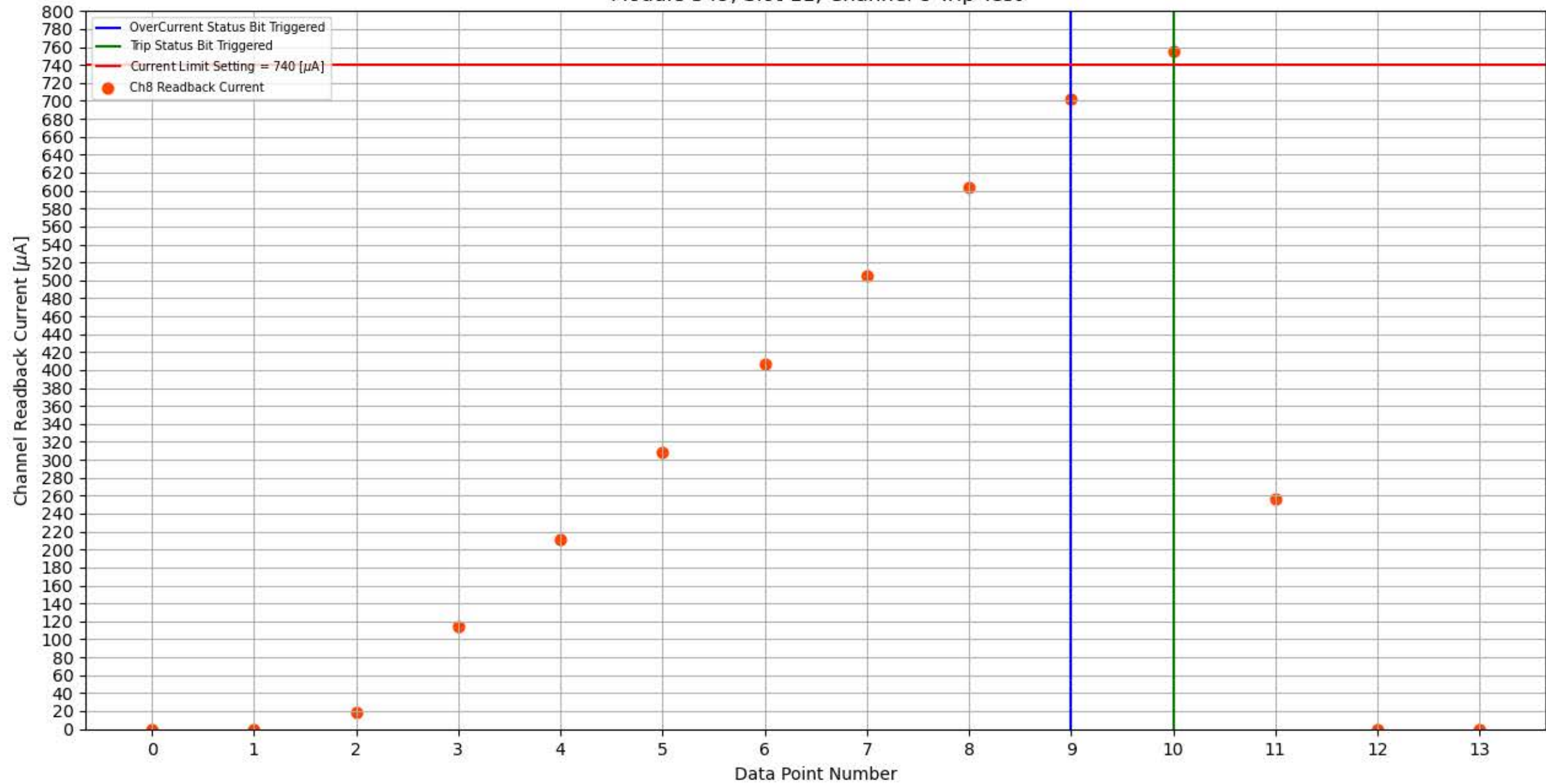
Module 349, Slot 11, Channel 8 Trip Test
