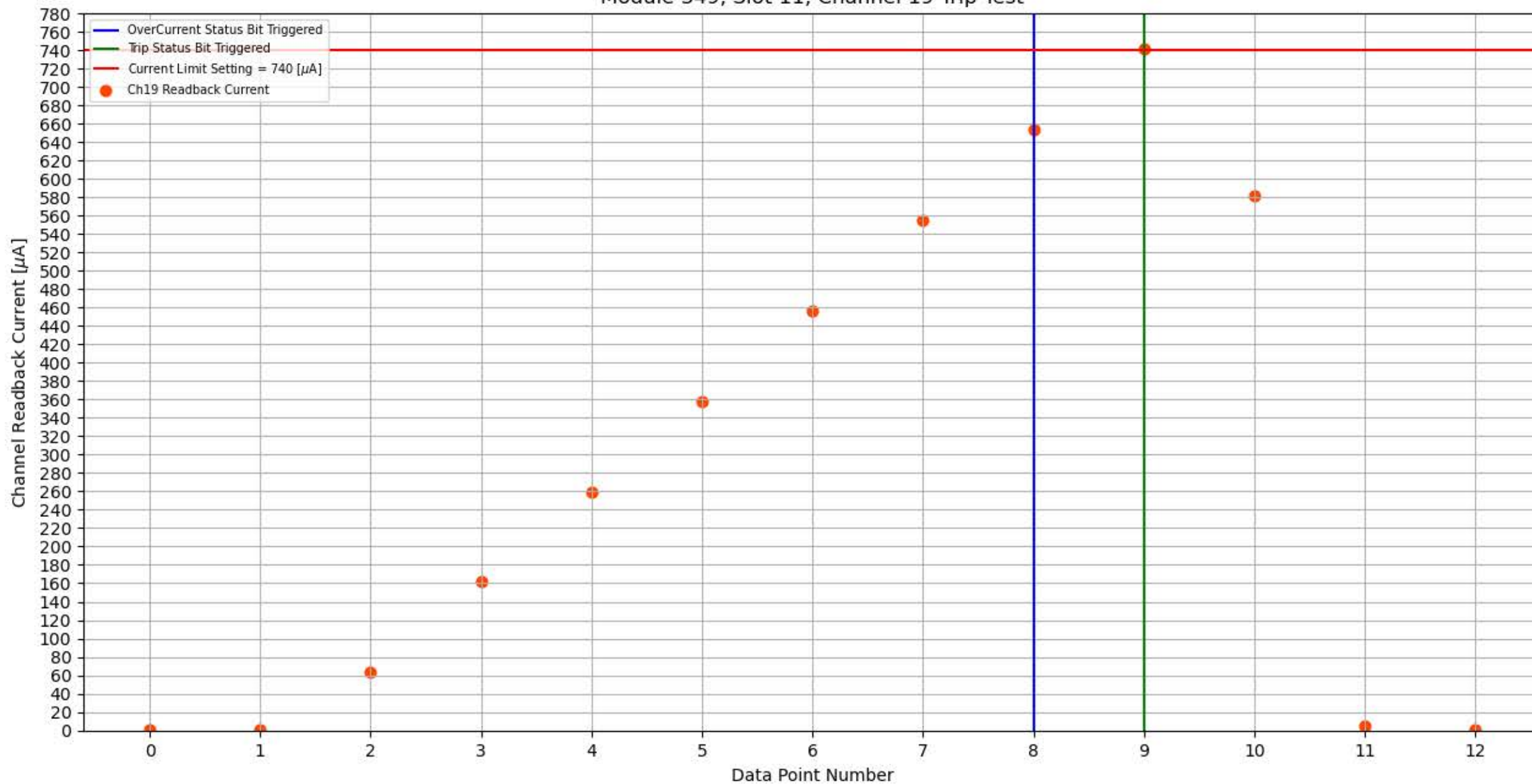
Module 349, Slot 11, Channel 19 Trip Test
