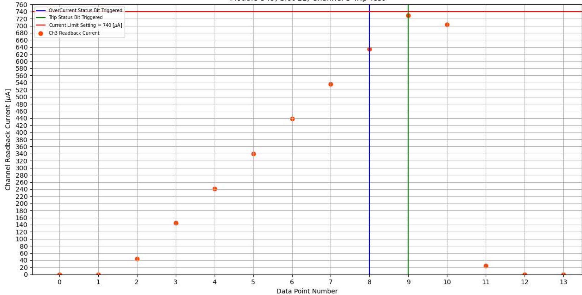
Module 349, Slot 11, Channel 3 Trip Test
