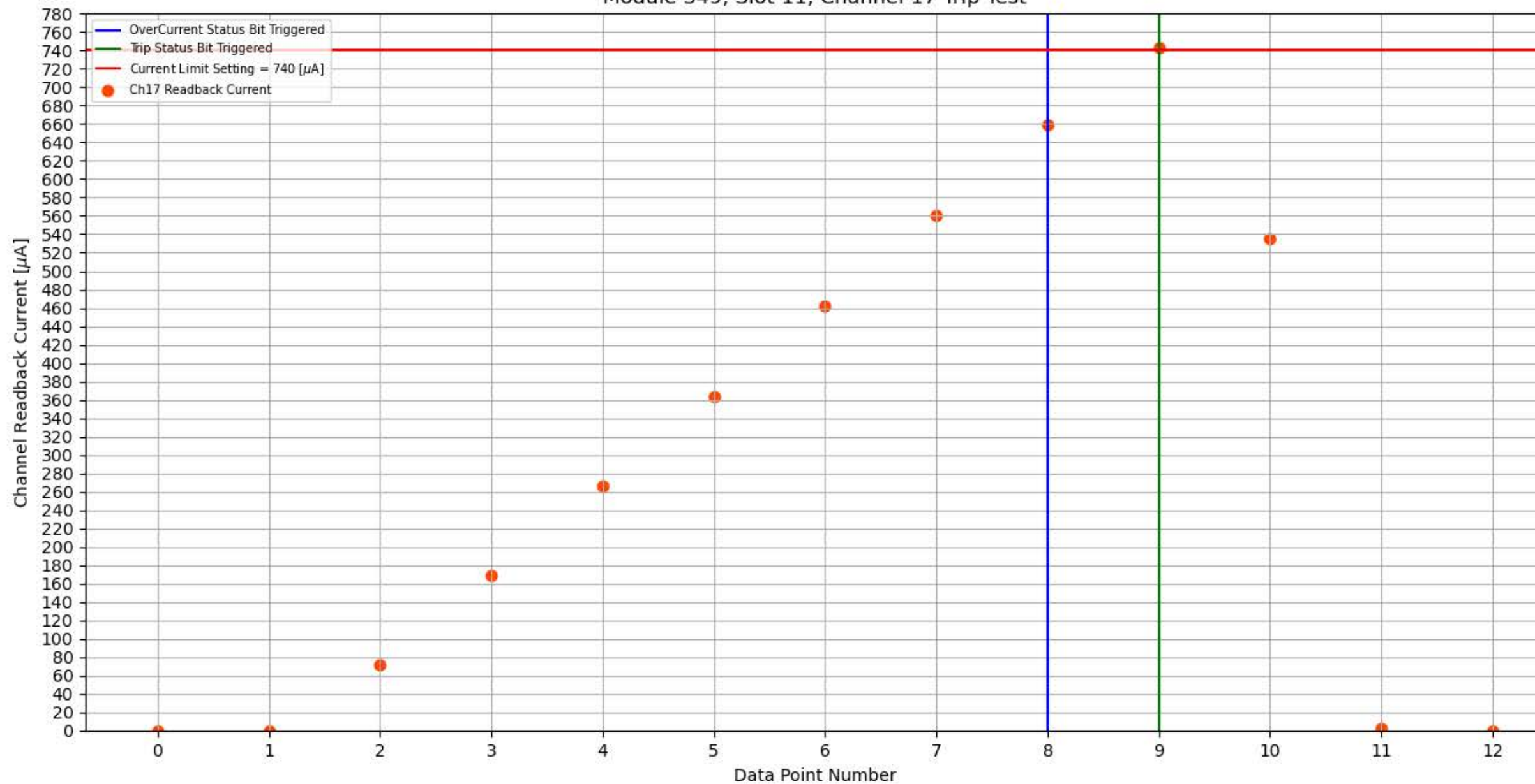
Module 349, Slot 11, Channel 17 Trip Test
