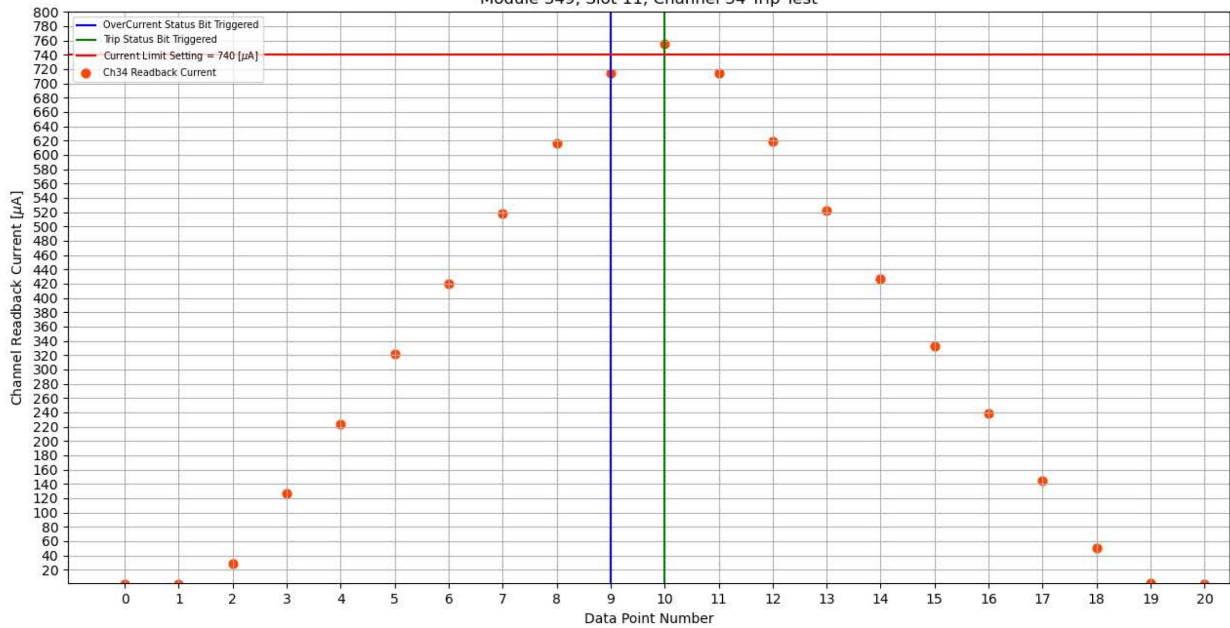
Module 349, Slot 11, Channel 34 Trip Test
