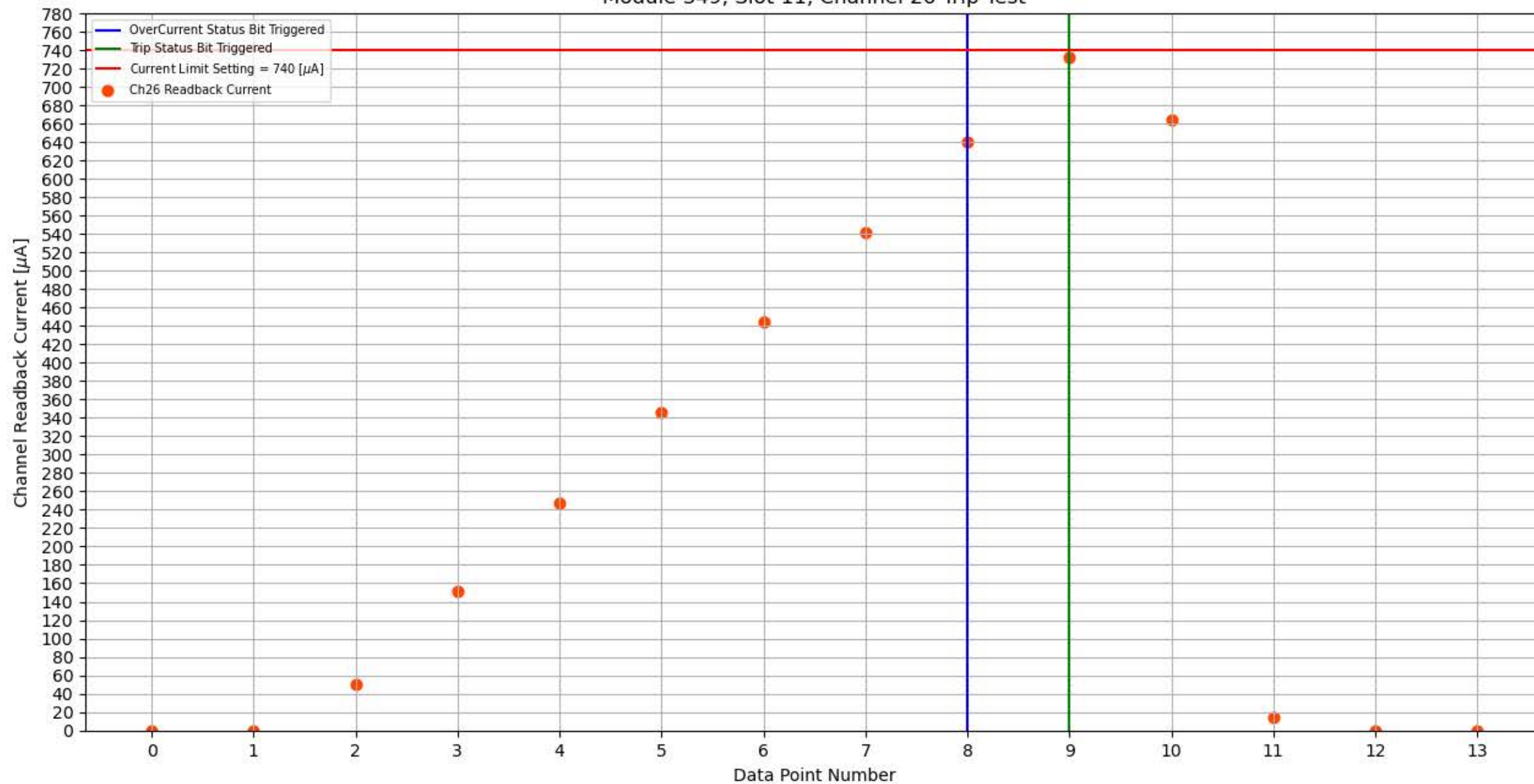
Module 349, Slot 11, Channel 26 Trip Test
