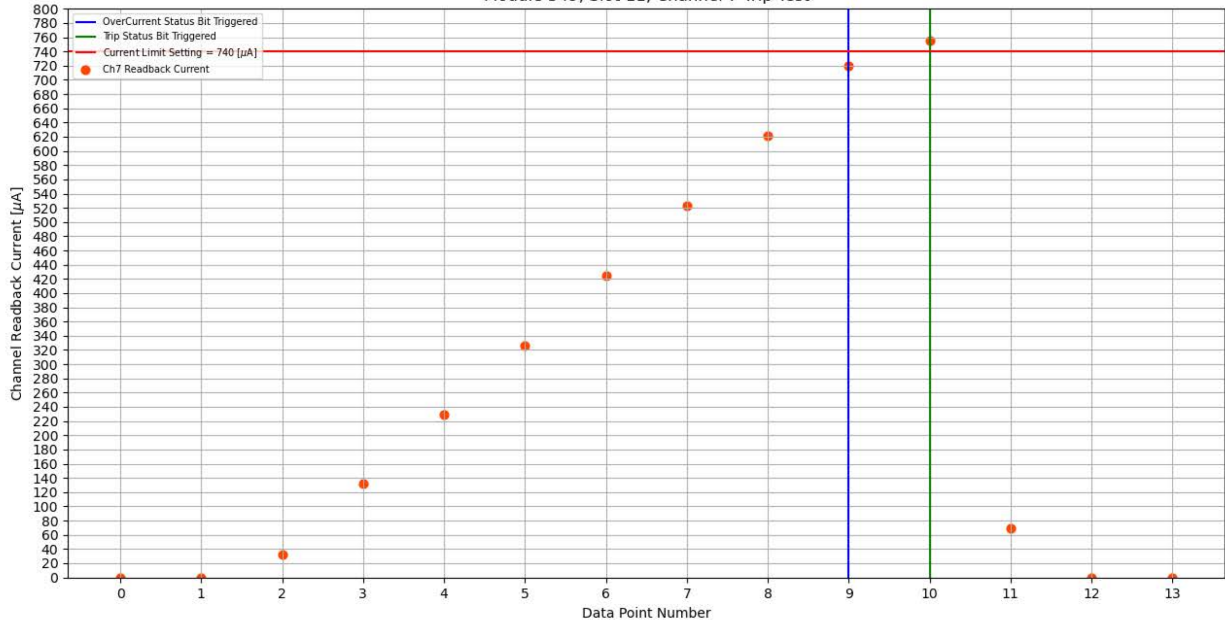
Module 349, Slot 11, Channel 7 Trip Test
