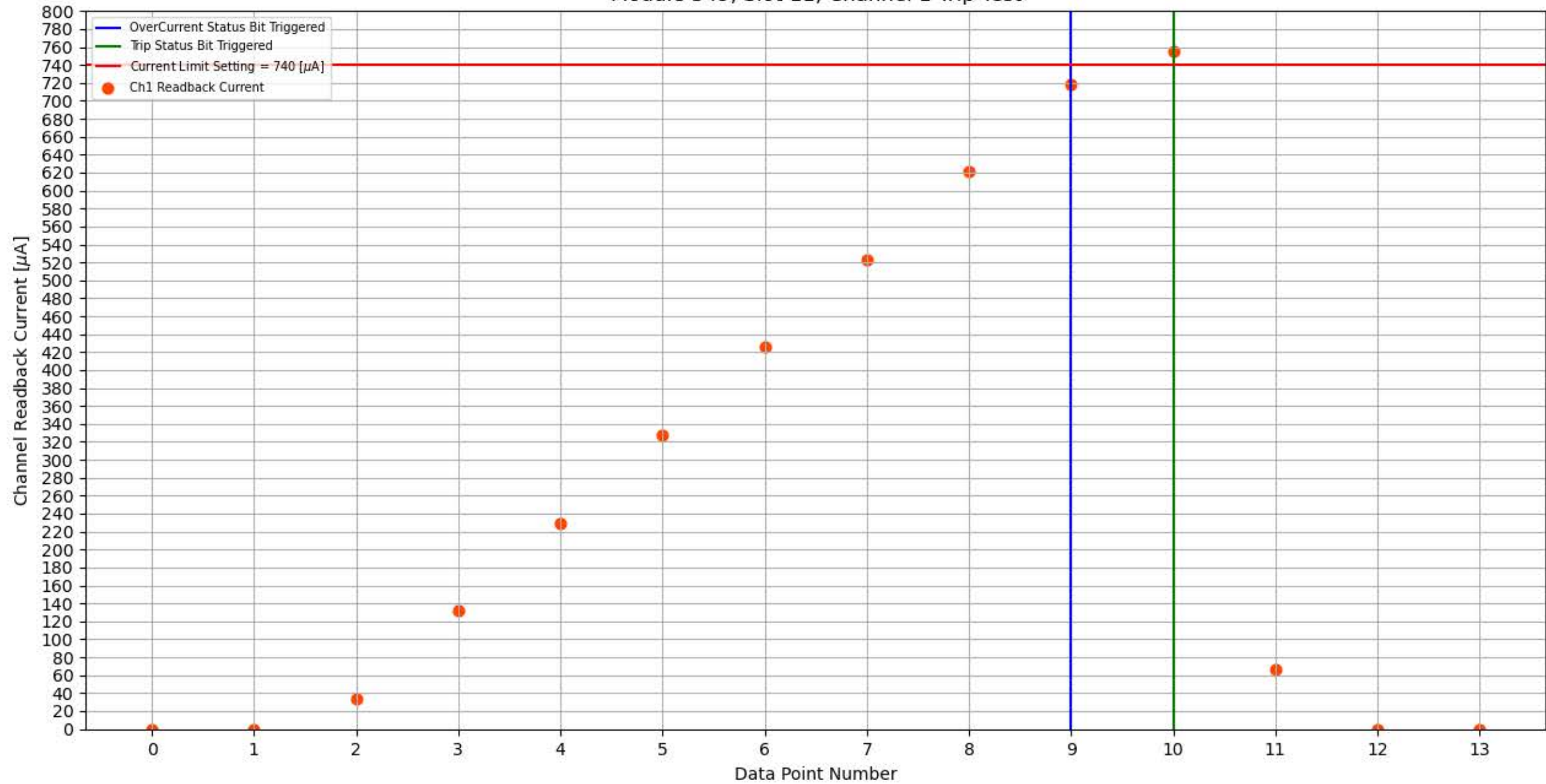
Module 349, Slot 11, Channel 1 Trip Test
