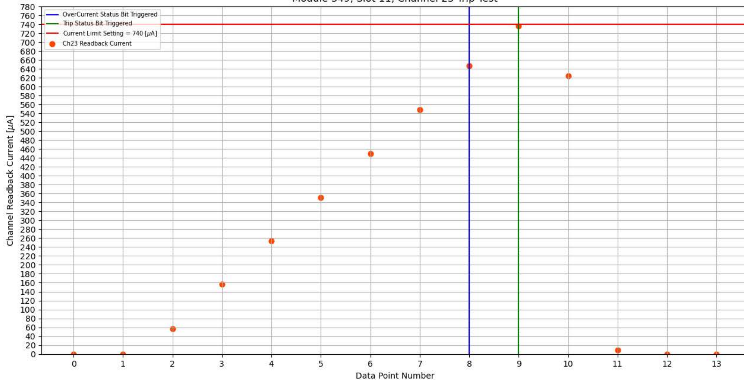
Module 349, Slot 11, Channel 23 Trip Test
