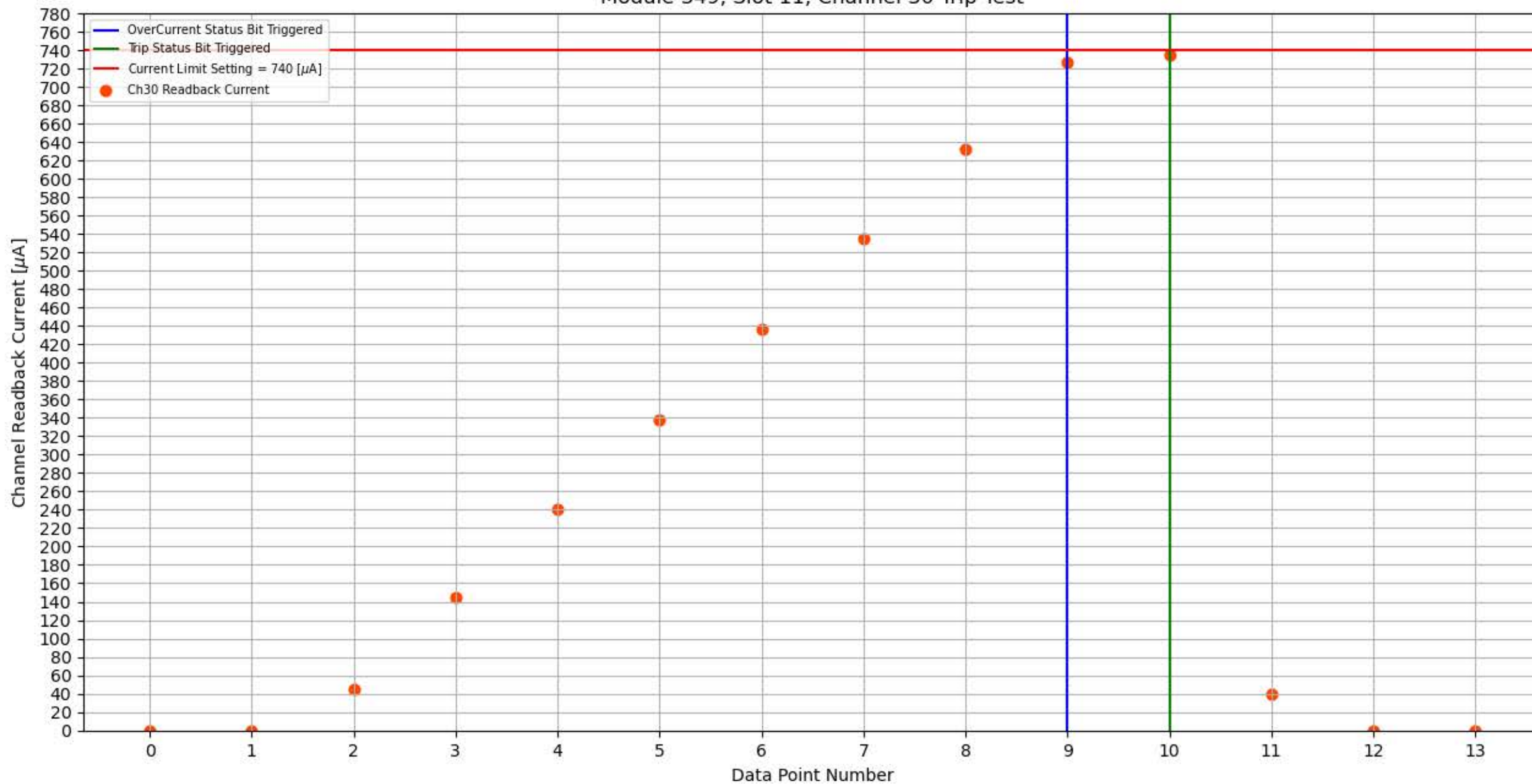
Module 349, Slot 11, Channel 30 Trip Test
