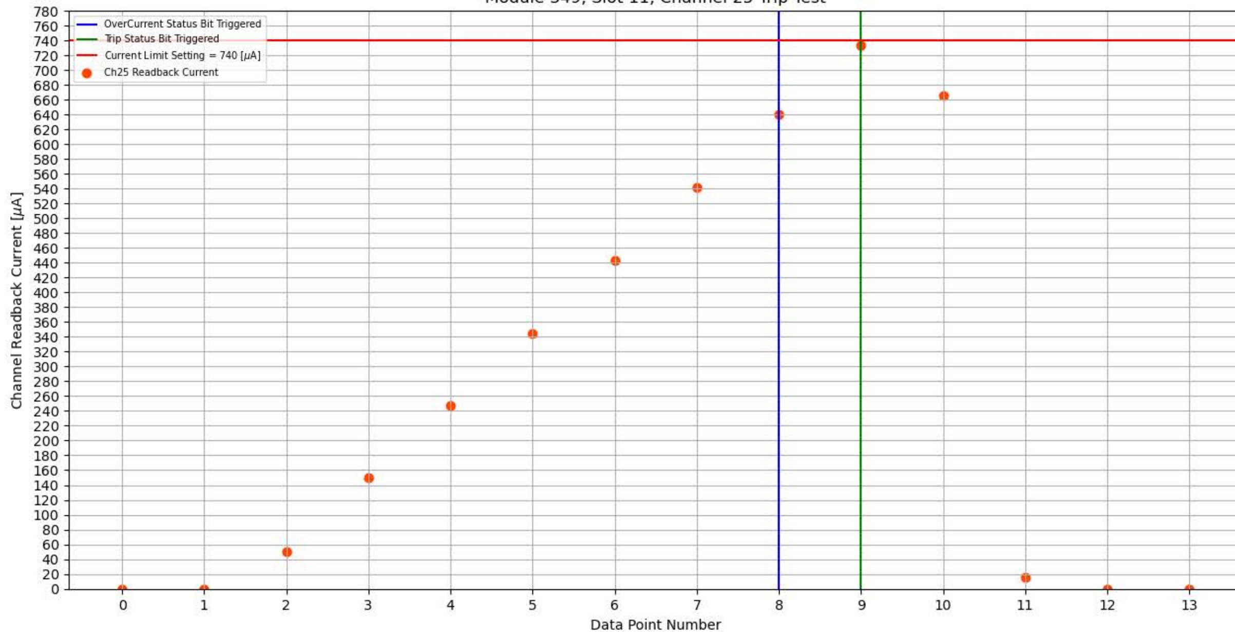
Module 349, Slot 11, Channel 25 Trip Test
