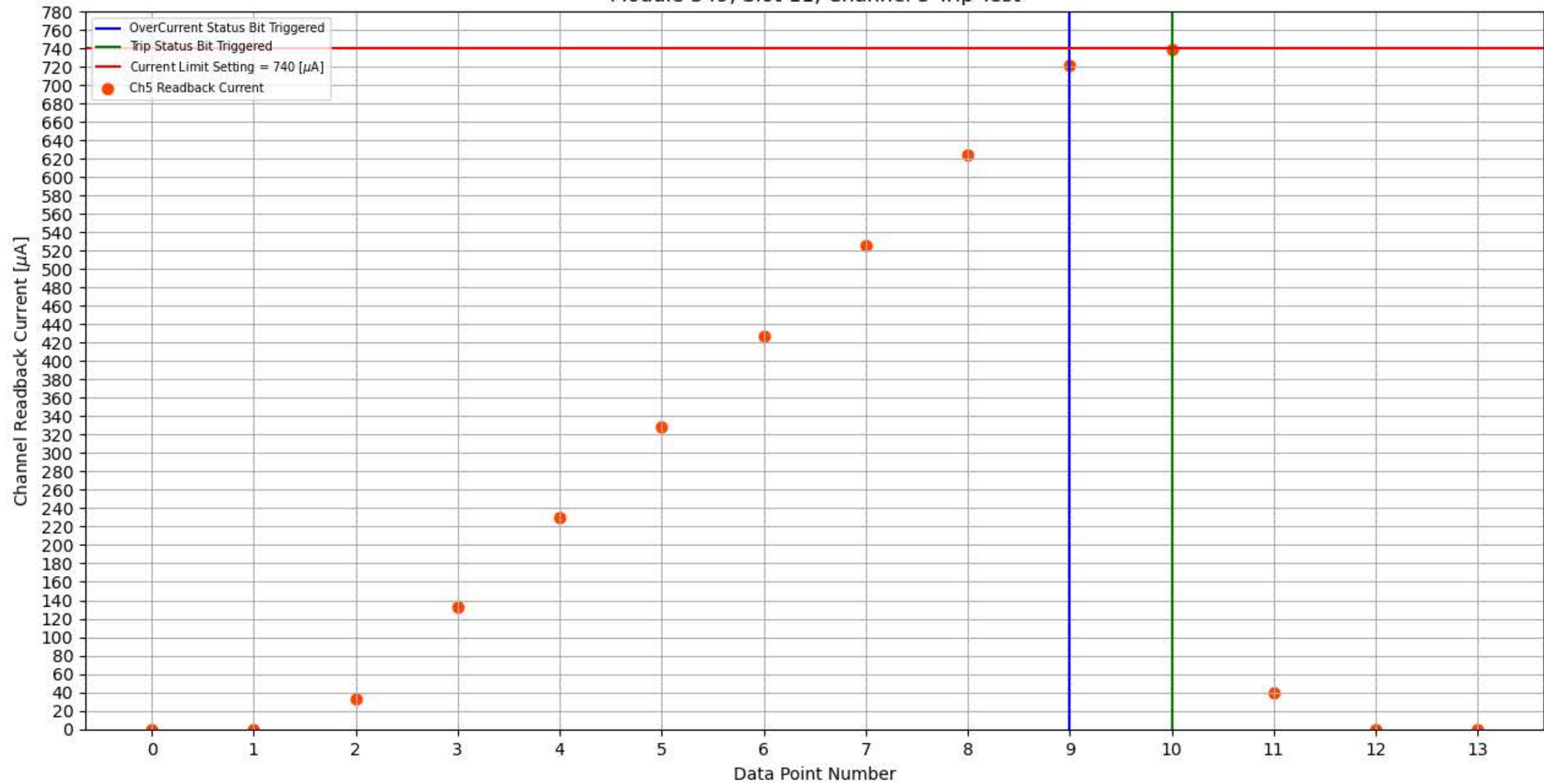
Module 349, Slot 11, Channel 5 Trip Test
