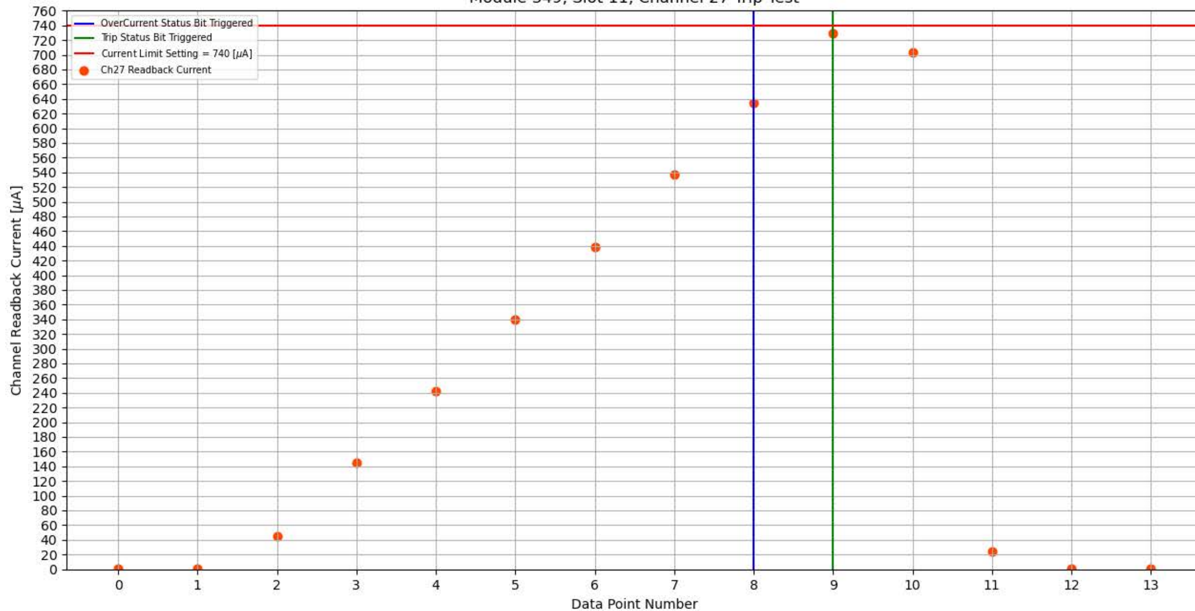
Module 349, Slot 11, Channel 27 Trip Test
