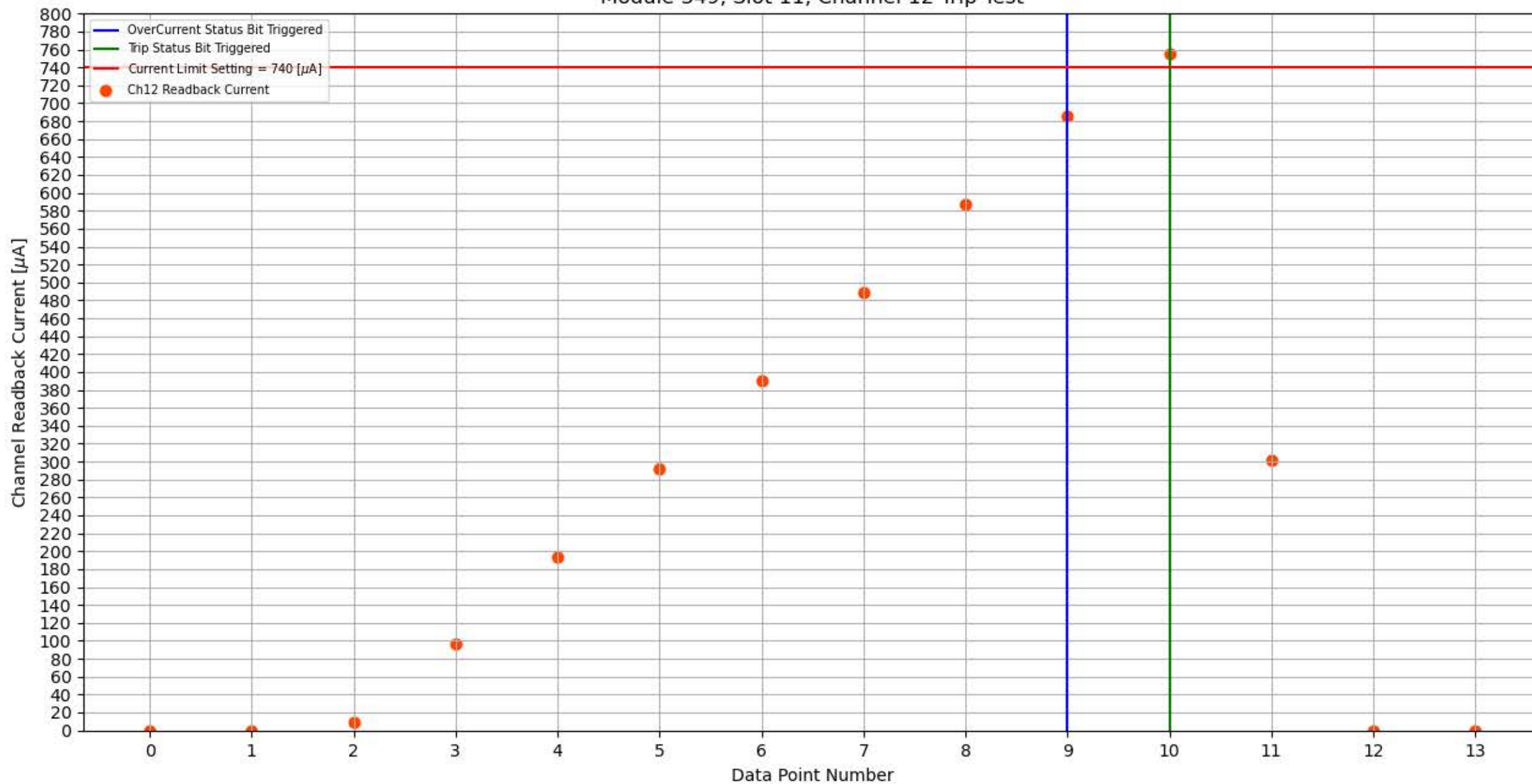
Module 349, Slot 11, Channel 12 Trip Test
