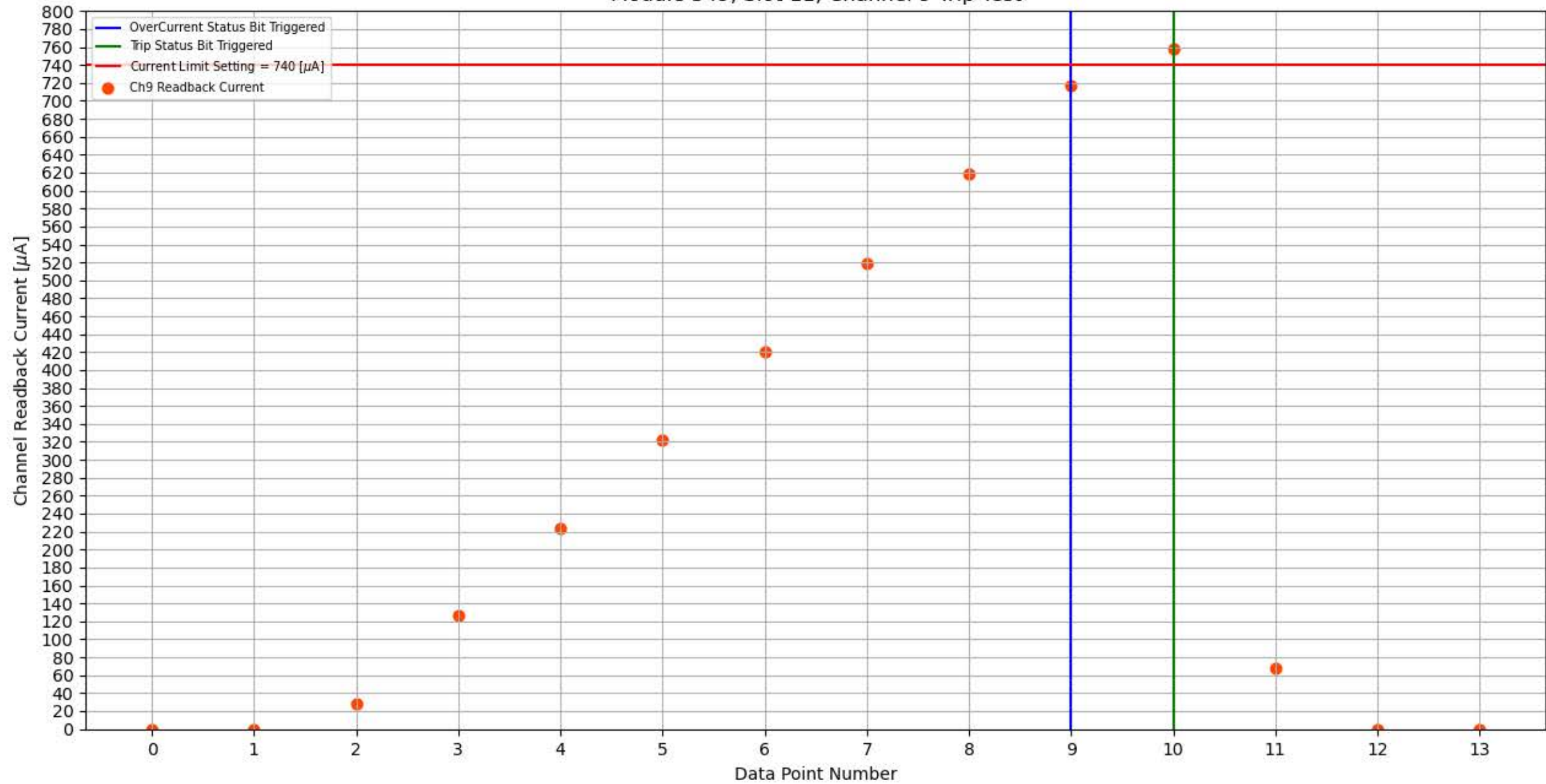
Module 349, Slot 11, Channel 9 Trip Test
