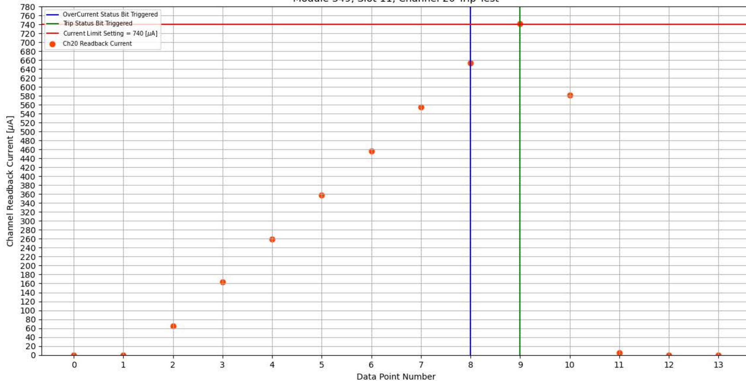
Module 349, Slot 11, Channel 20 Trip Test
