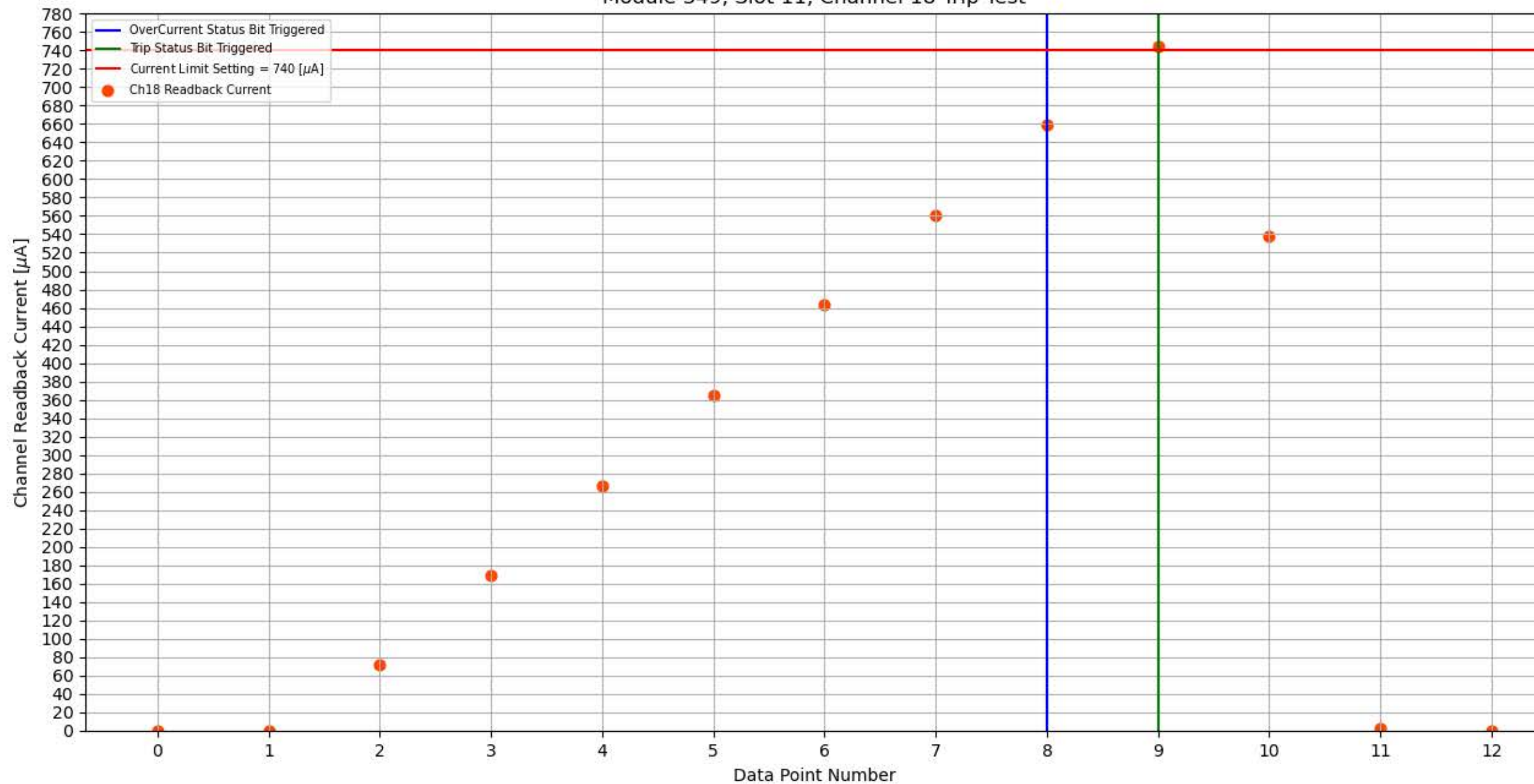
Module 349, Slot 11, Channel 18 Trip Test
