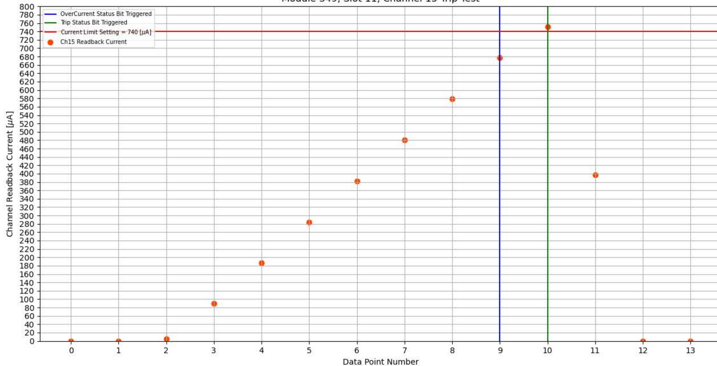
Module 349, Slot 11, Channel 15 Trip Test
