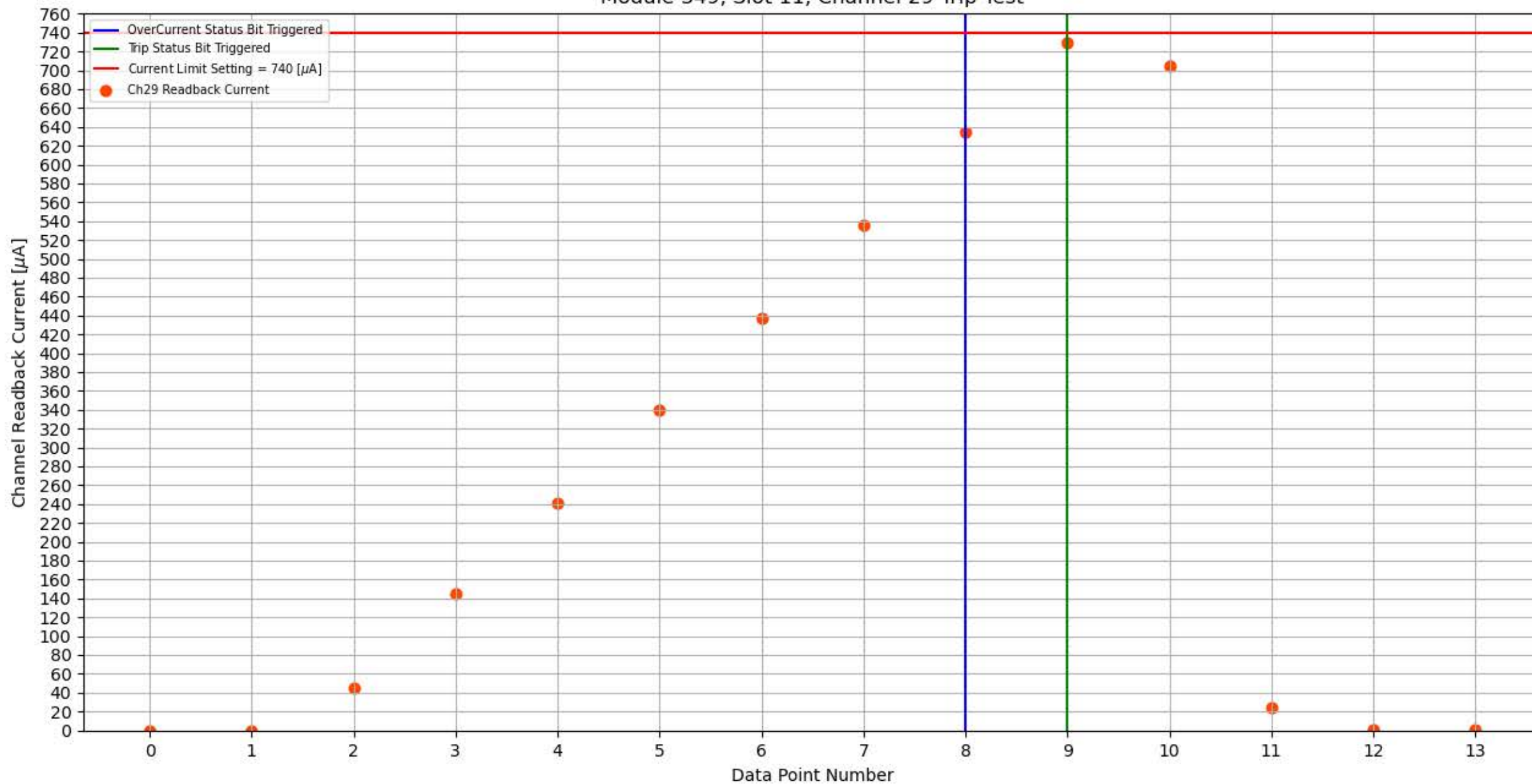
Module 349, Slot 11, Channel 29 Trip Test
