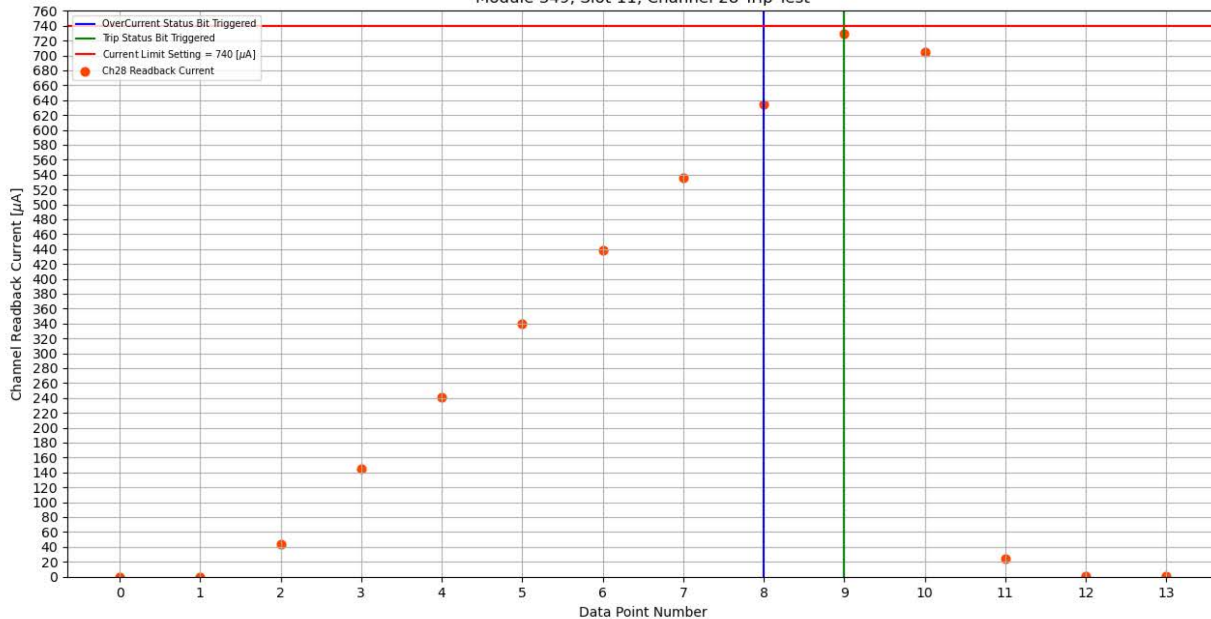
Module 349, Slot 11, Channel 28 Trip Test
