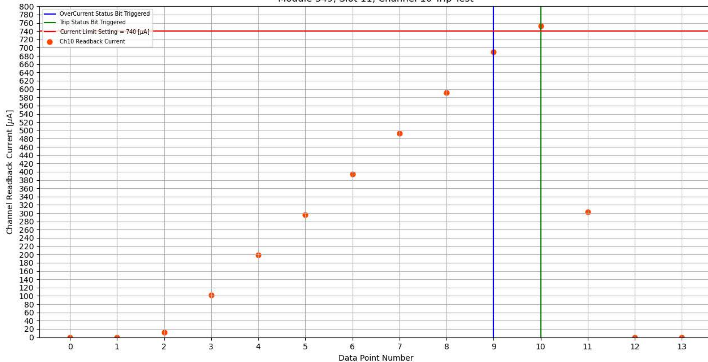
Module 349, Slot 11, Channel 10 Trip Test
