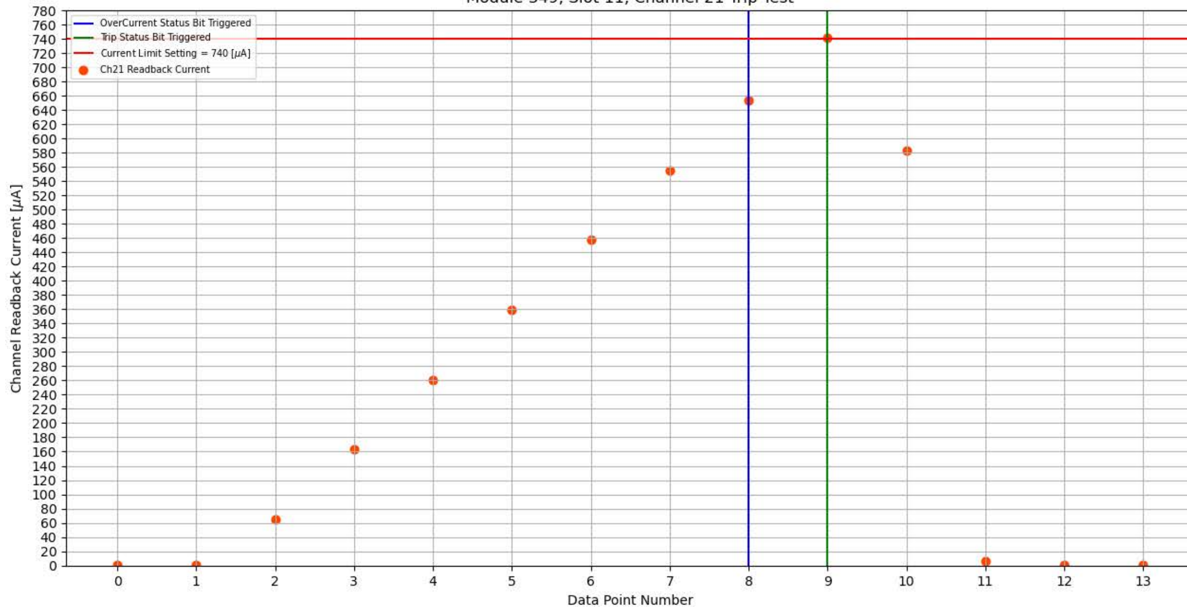
Module 349, Slot 11, Channel 21 Trip Test
