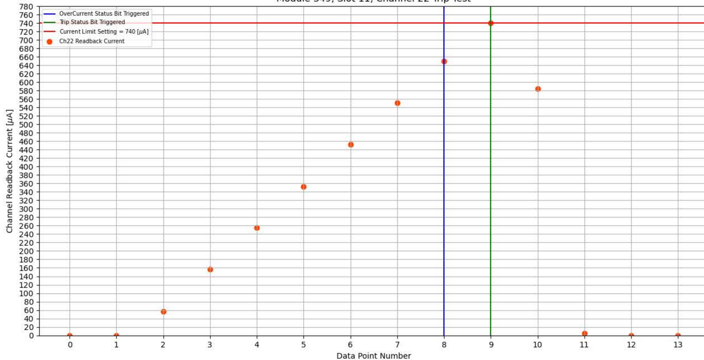
Module 349, Slot 11, Channel 22 Trip Test
