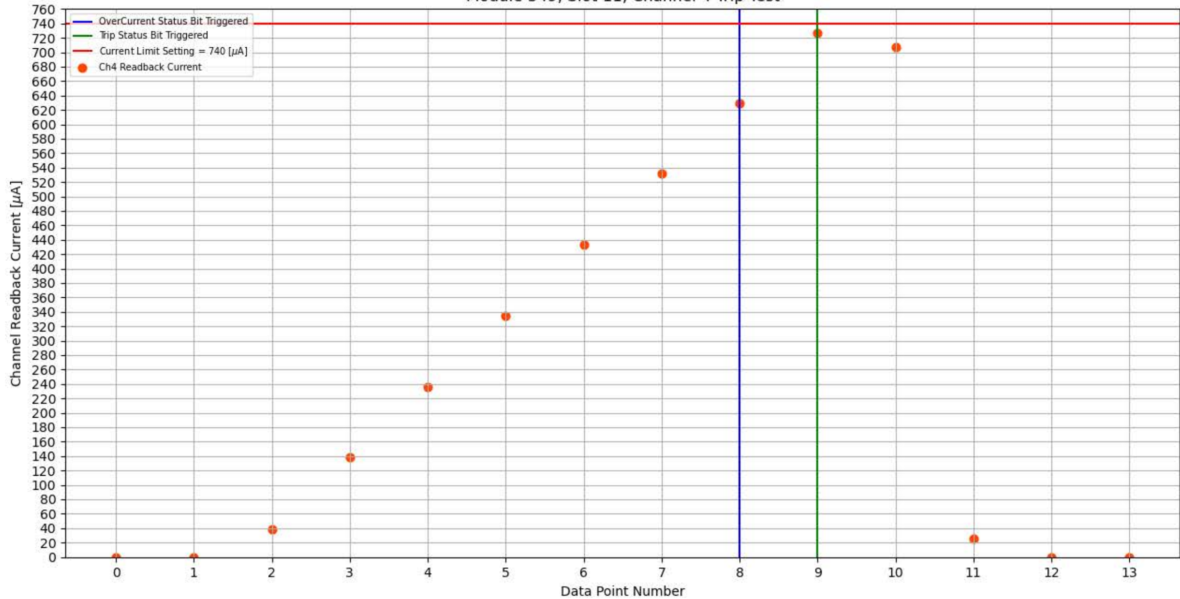
Module 349, Slot 11, Channel 4 Trip Test
