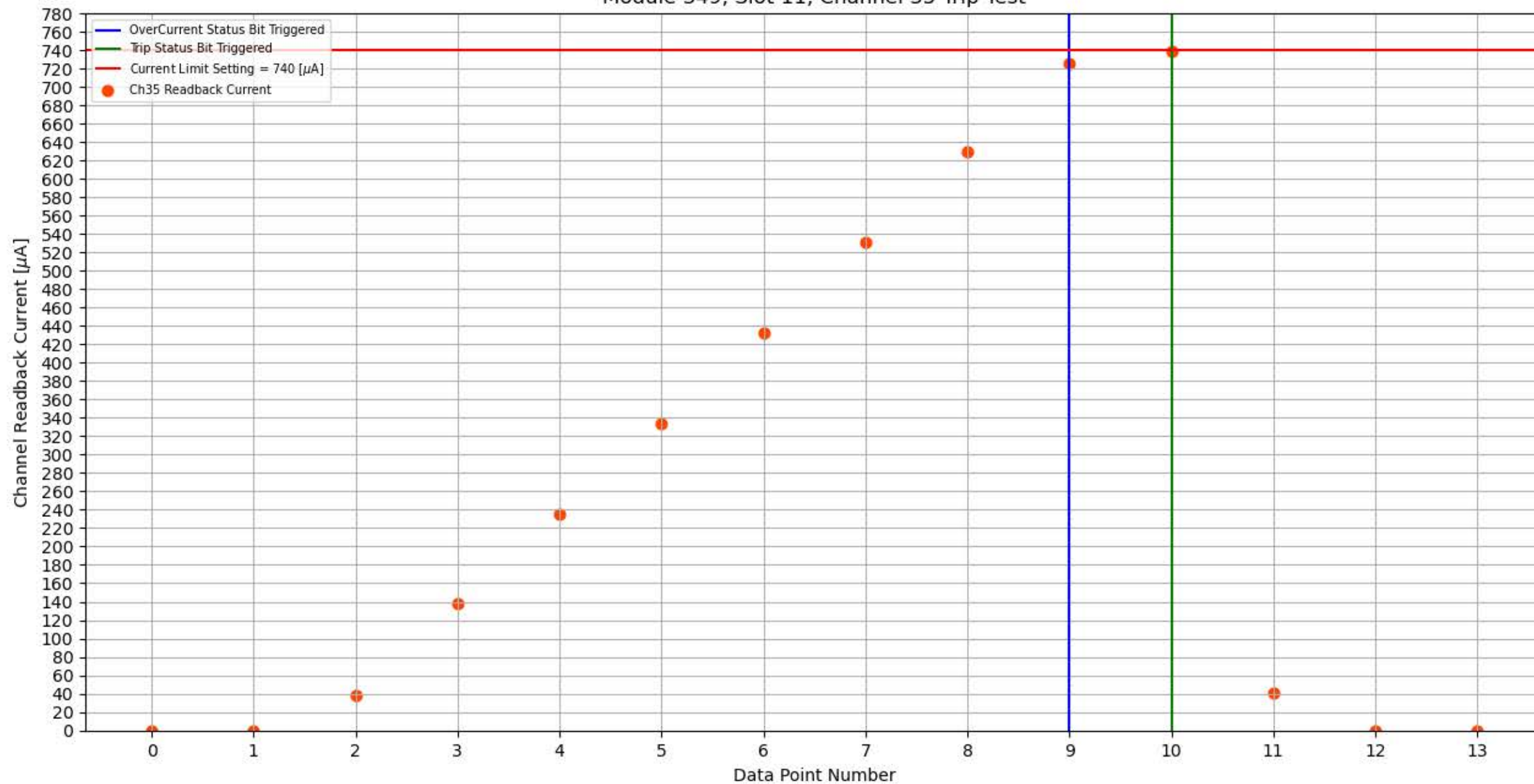
Module 349, Slot 11, Channel 35 Trip Test
