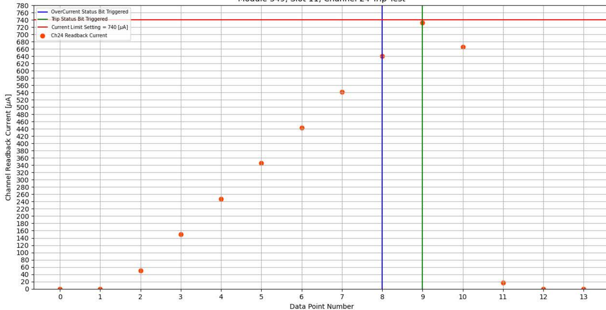
Module 349, Slot 11, Channel 24 Trip Test
