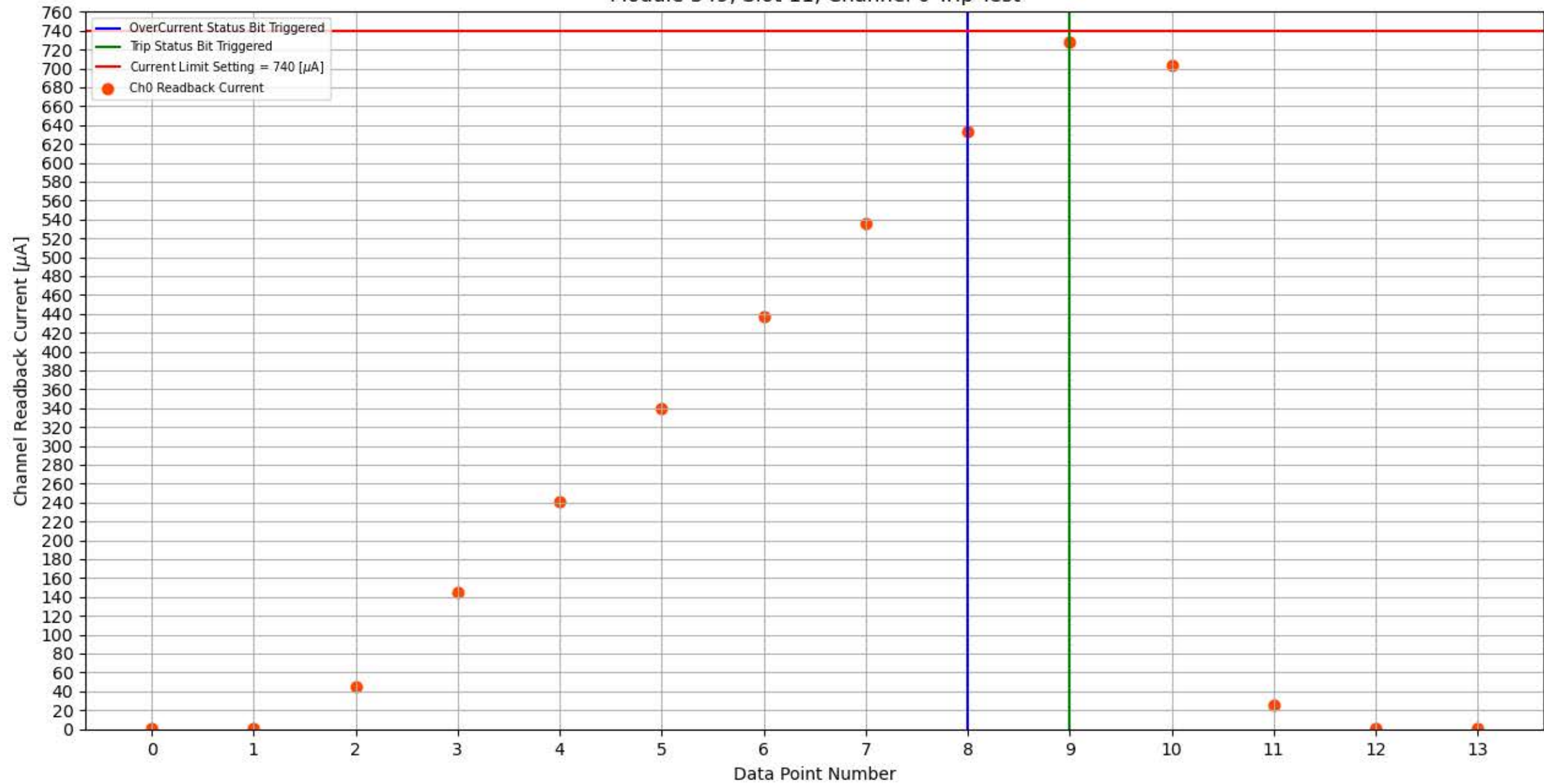
Module 349, Slot 11, Channel 0 Trip Test
